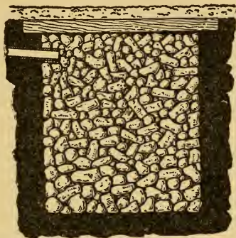
Fig. 52.—Soak-away drain
